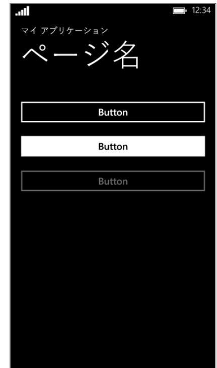
Windows Phone8
