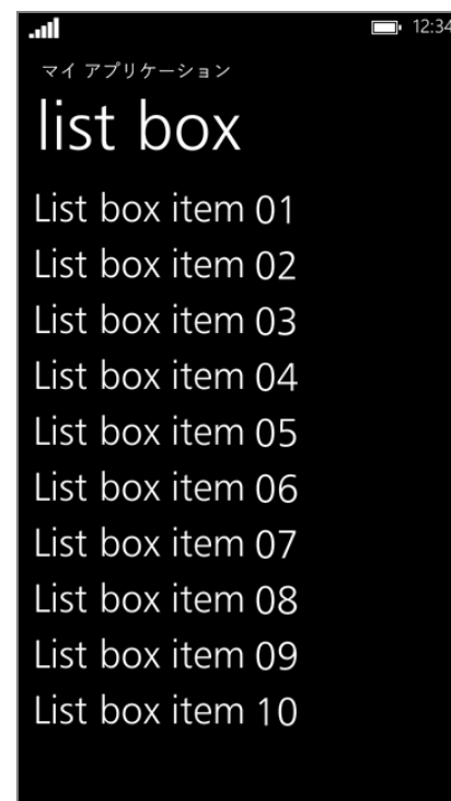
Windows Phone8
