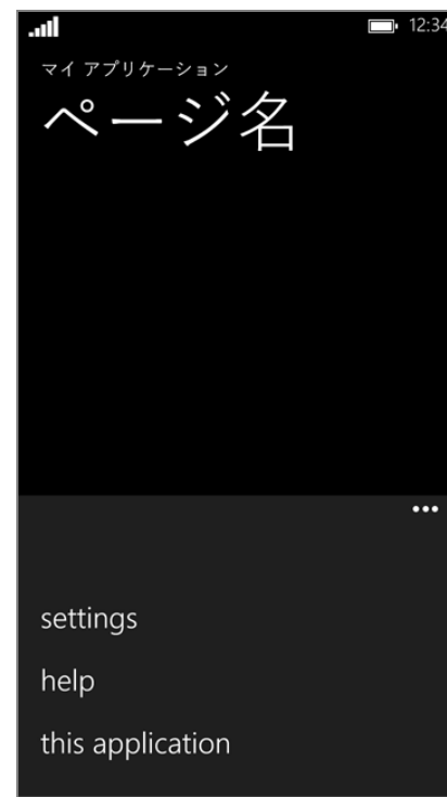
Windows Phone8
