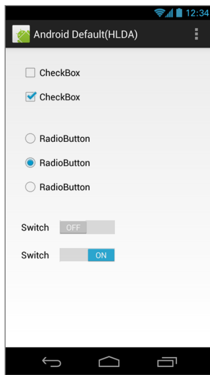
Android 4.2
