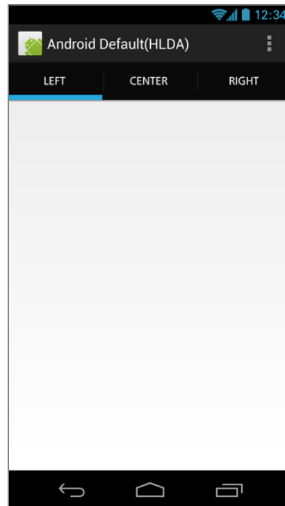
Android 4.2
