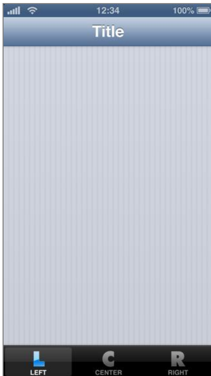
iOS
