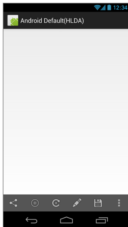
Android 4.2
